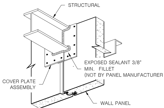
PENETRATION PERIMETER SEAL
