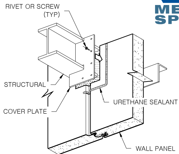
RIGHT COVER PLATE INSTALLATION
