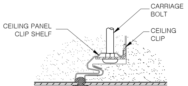
Panel Joint Section
