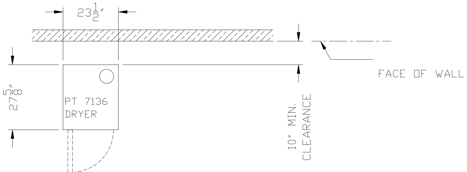
PLAN VIEW
