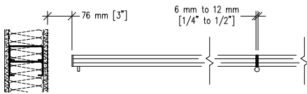
No closure
