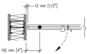
Pivot closure
