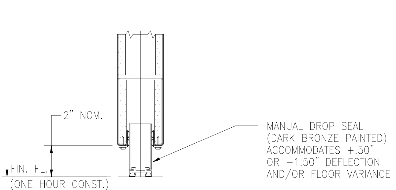
VERTICAL SECTION
