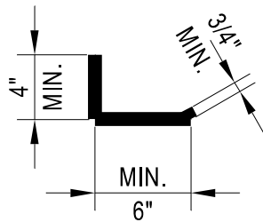
MINIMUM PAN FLASHING
