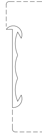
Exposed Surfaces Scale 1 : 1
