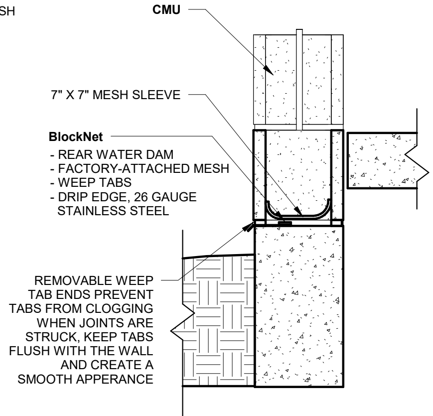
SECTION VIEW
