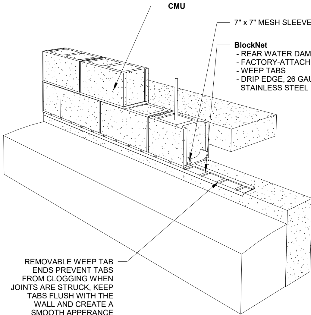
PERSPECTIVE VIEW
