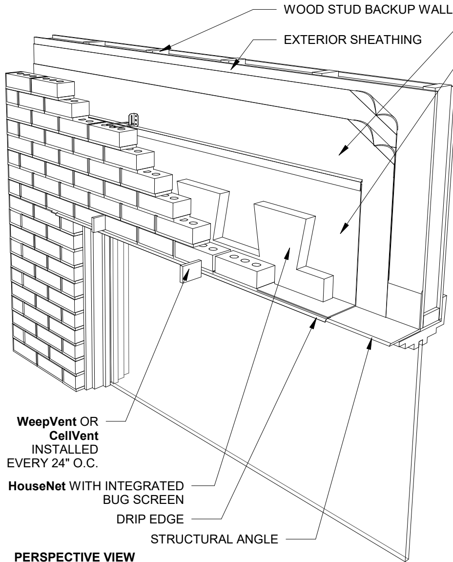
PERSPECTIVE VIEW
