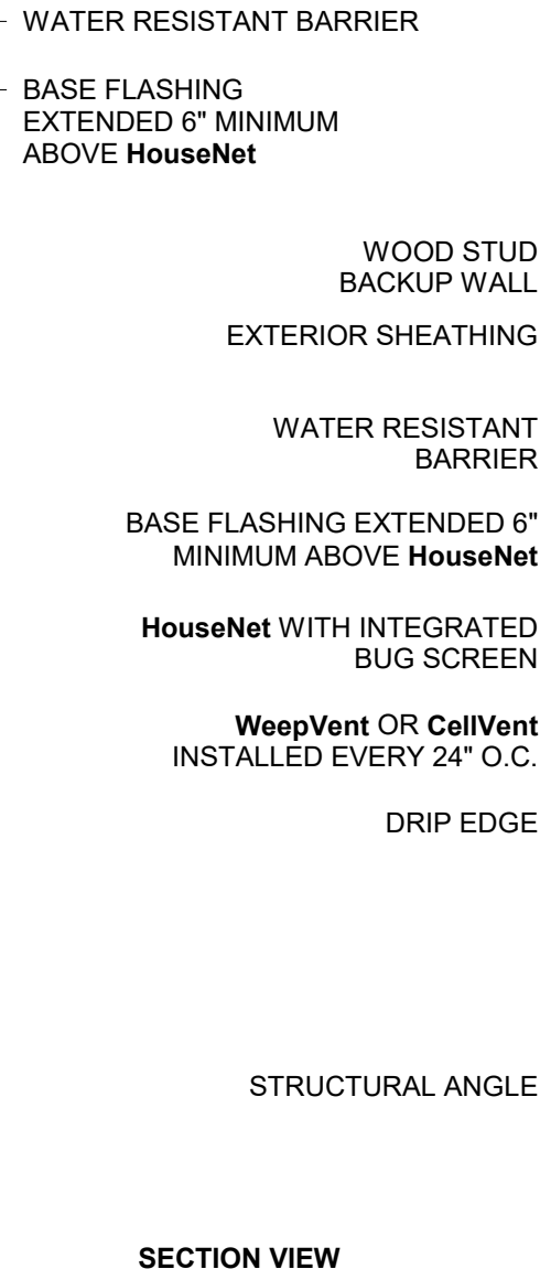
SECTION VIEW
