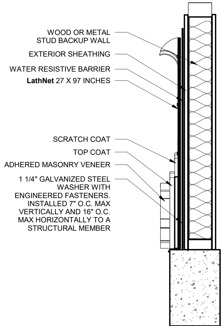
SECTION VIEW
