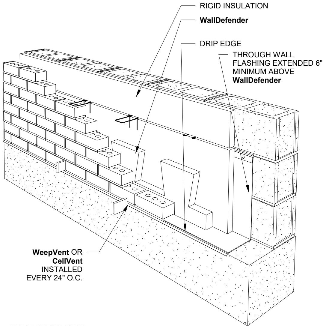
PERSPECTIVE VIEW
