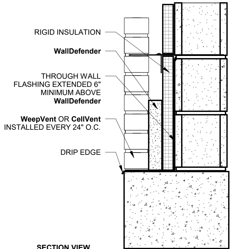
SECTION VIEW
