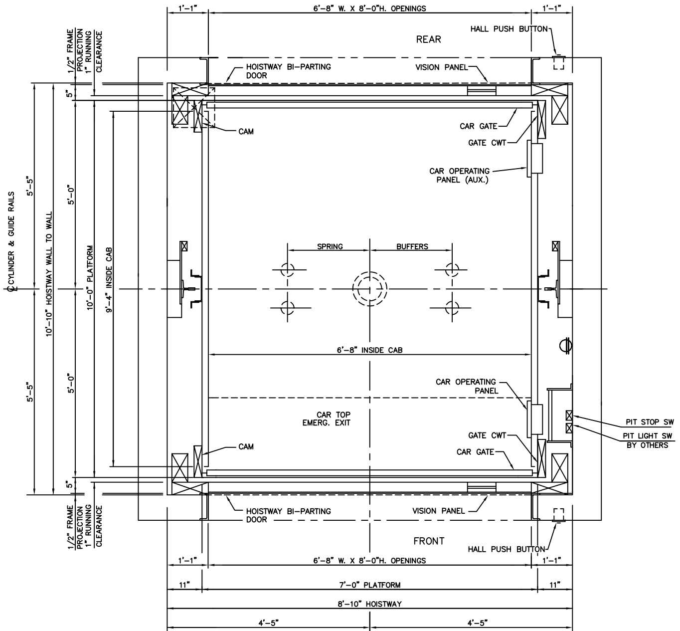
CYLINDER & PLATFORM HOISTWAY PLAN
