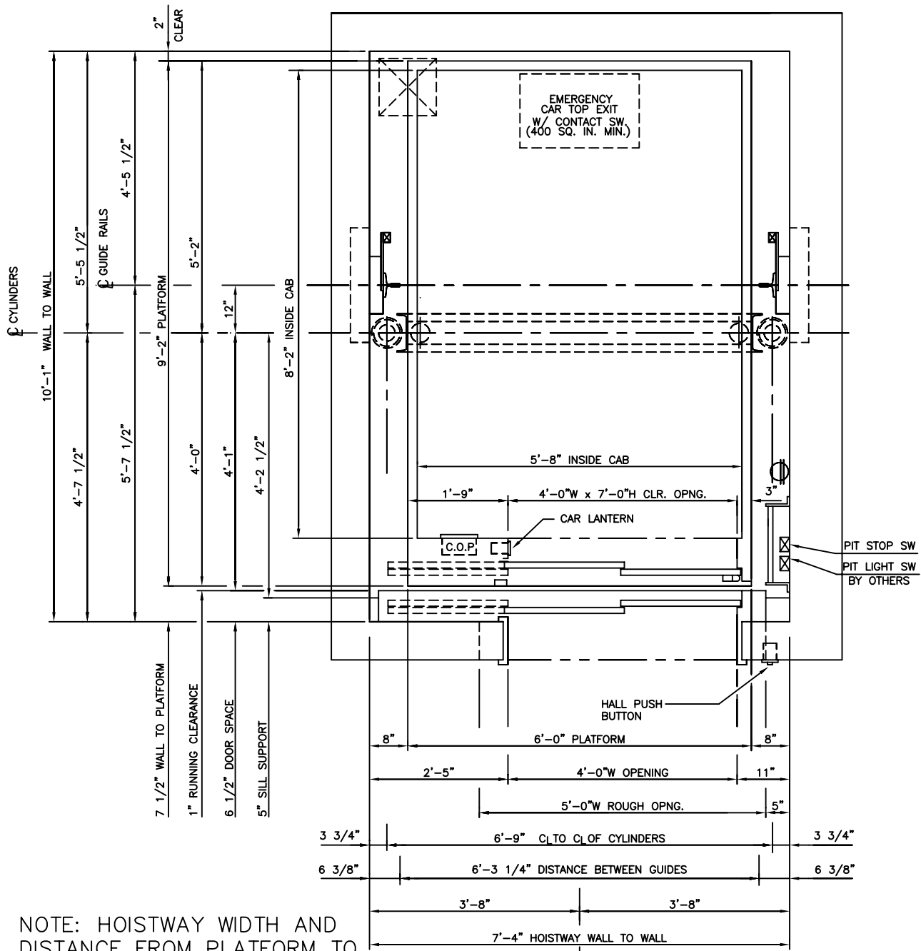
HOISTWAY PLAN ALL DIMENSIONS ARE SUBJECT TO CHANGE WITHOUT NOTICE. CONSULT NATIONWIDE LIFTS CO. FOR CONFIRMATION.
