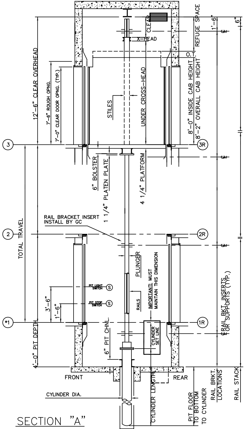
ELEVATION PLAN
