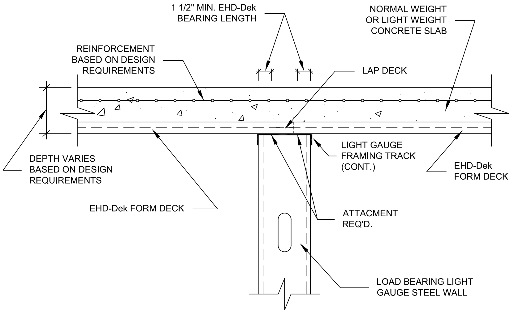
EHD-Dek ON LOAD BEARING LIGHT GAUGE STEEL WALL @ INTERIOR CONDITION
