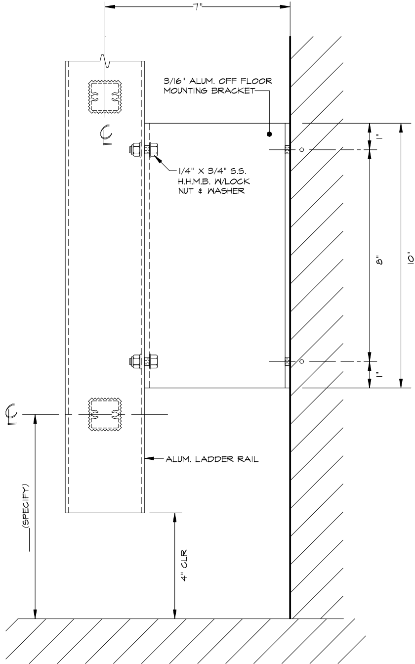
OFF FLOOR MOUNTING BRACKET SCALE: 3"=1'-0"
