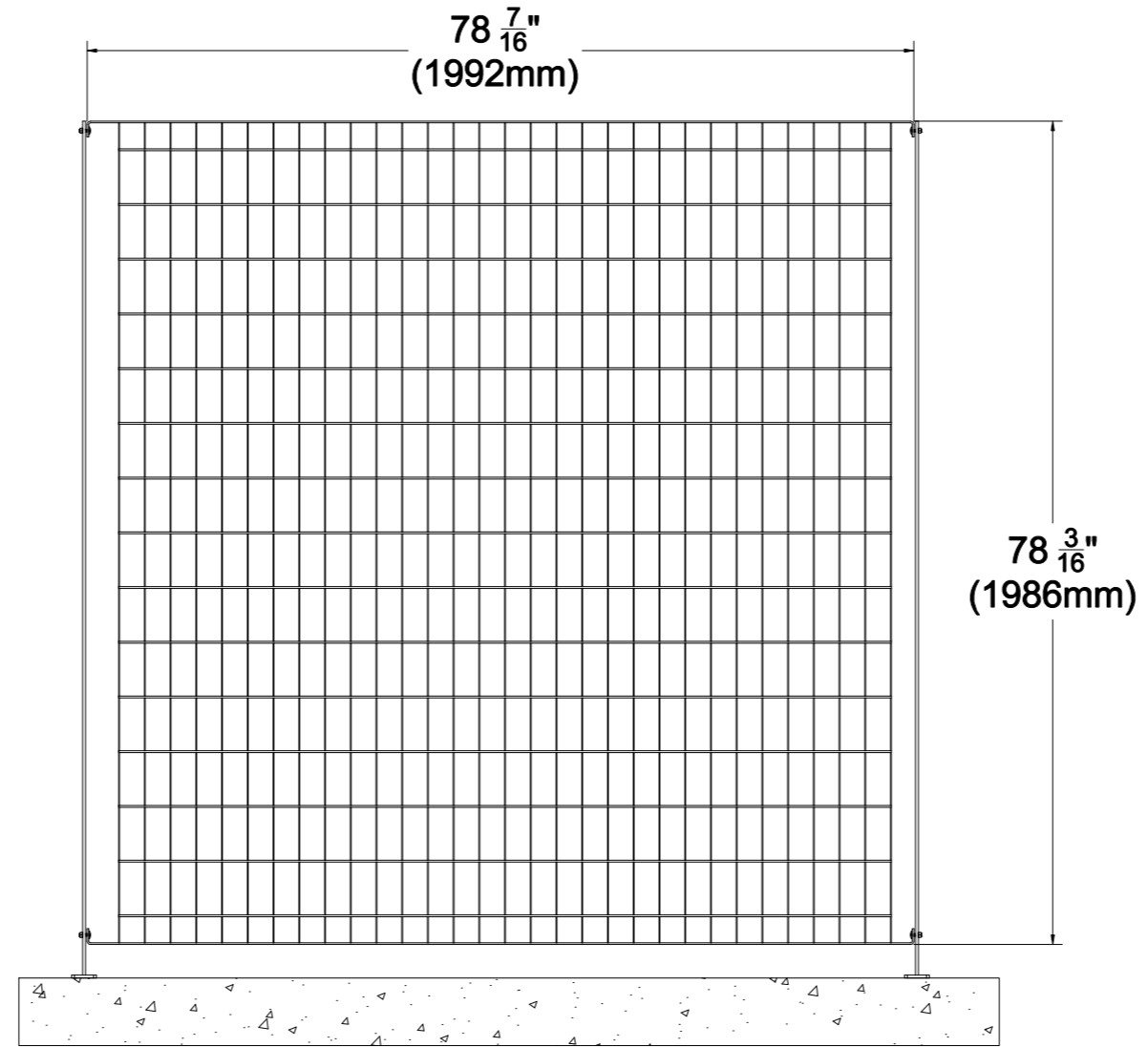
PANEL 6.5'H ON FLAT POSTS
