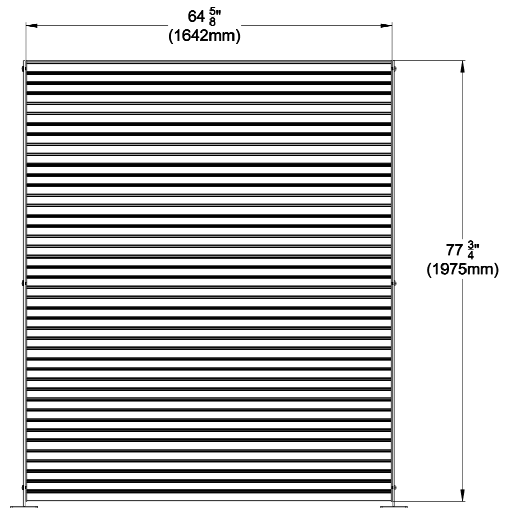
PANEL 6.5'H ON FLAT POSTS
