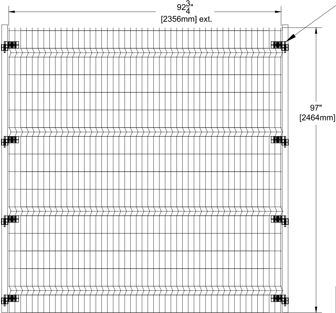
Panel 8'H (57 lbs/25.9 kg)
