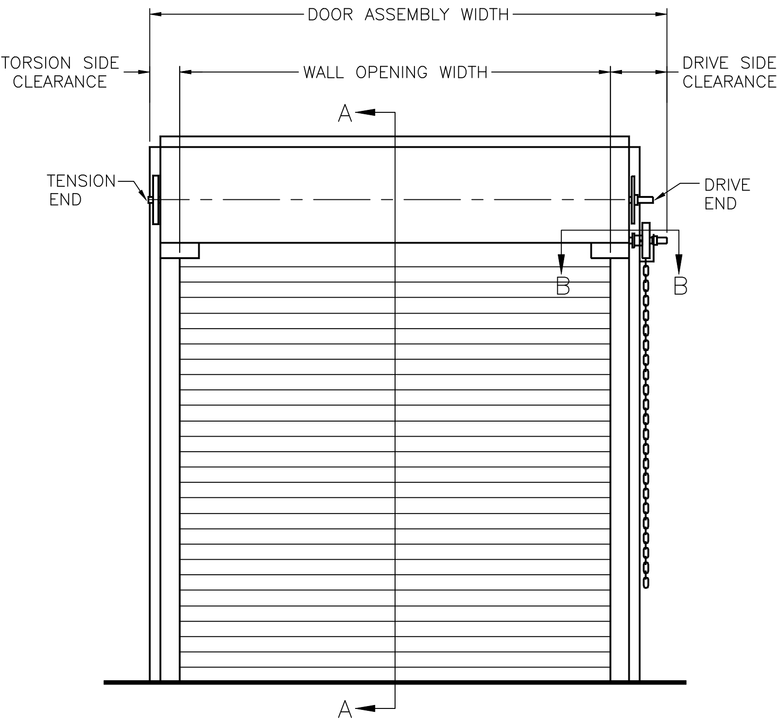
SERIES 600 HOIST OPERATED DOORS FACE-OF-WALL MOUNTED
