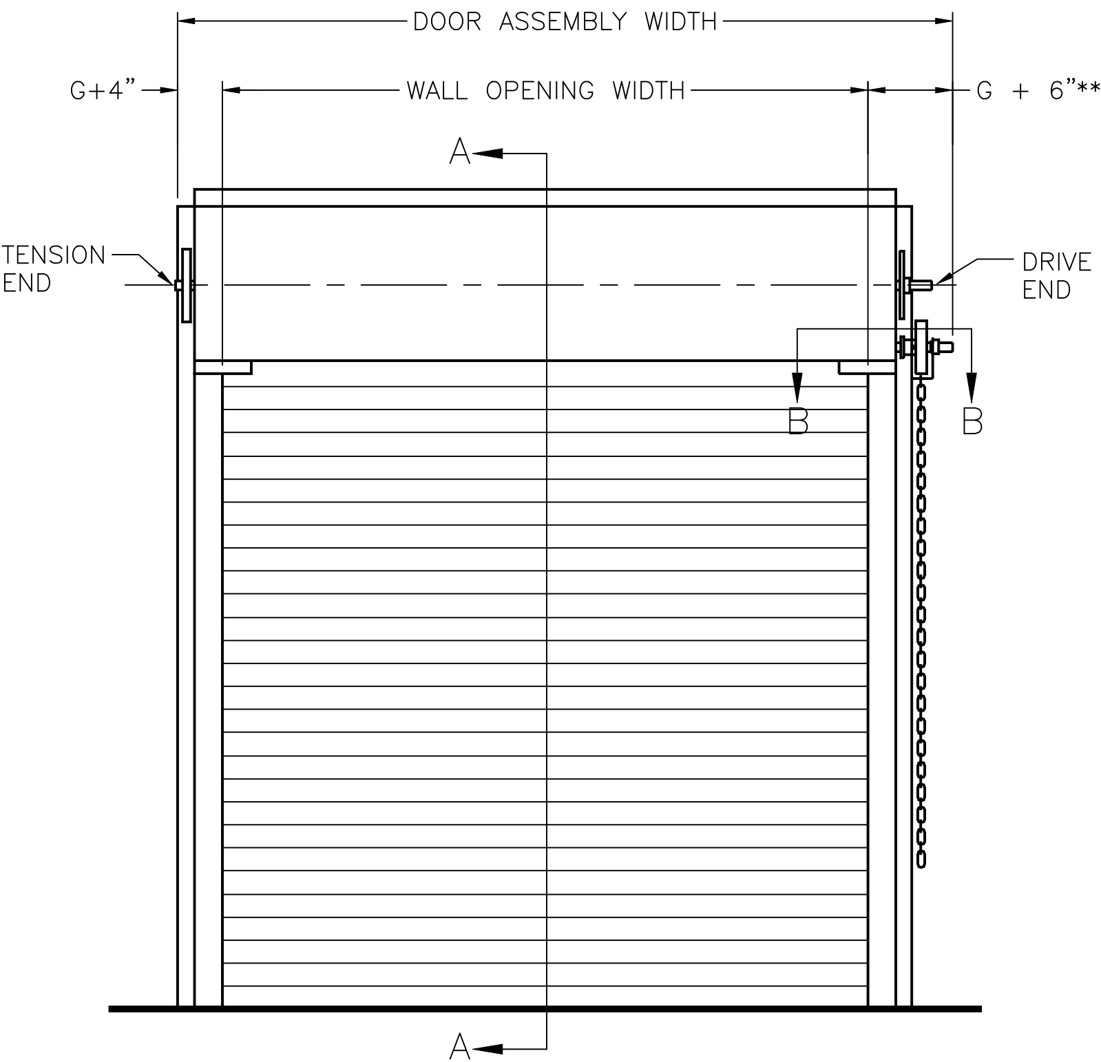
INSIDE FACE-OF-WALL MOUNTED CHAIN HOIST / MANUAL PUSH-UP RIGHT HAND OPERATION SHOWN - LEFT HAND OPPOSITE
