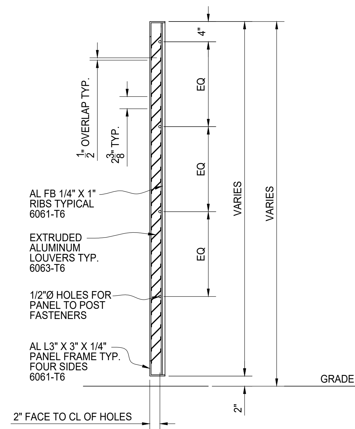
TYPICAL PANEL SECTION
