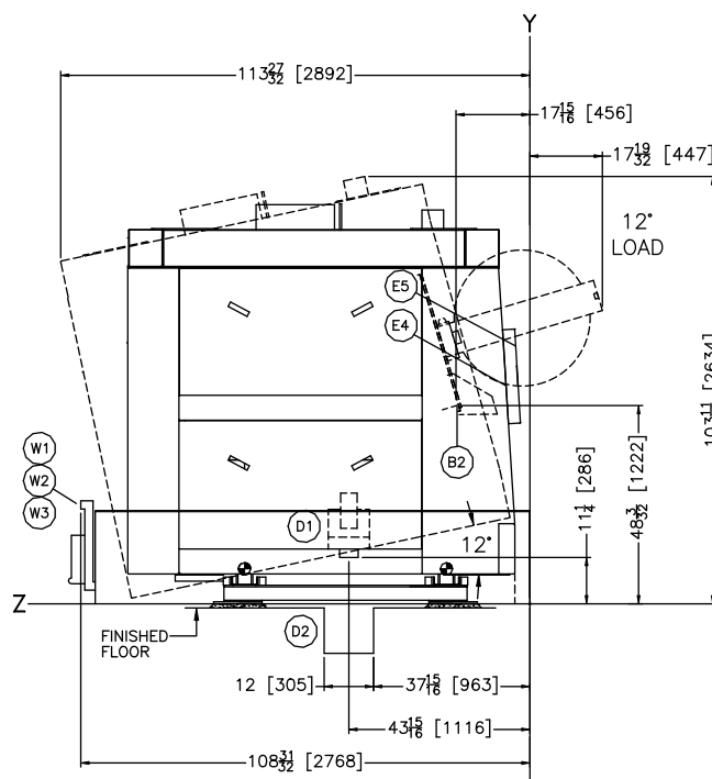
LEFT VIEW
