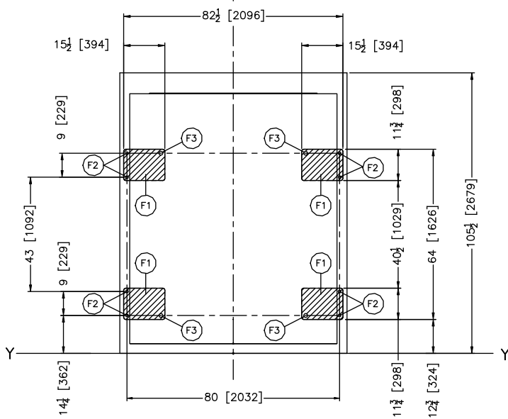
FOUNDATION VIEW
