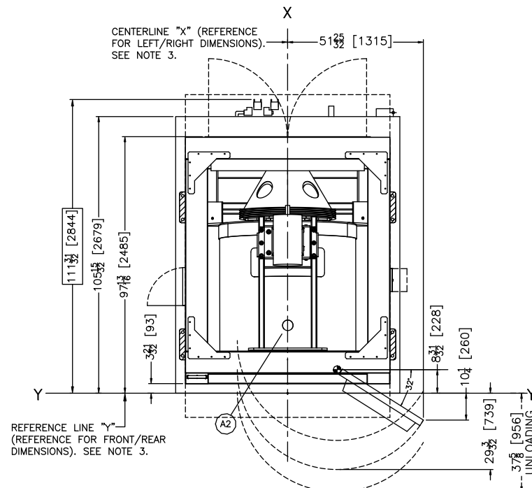
PLAN VIEW
