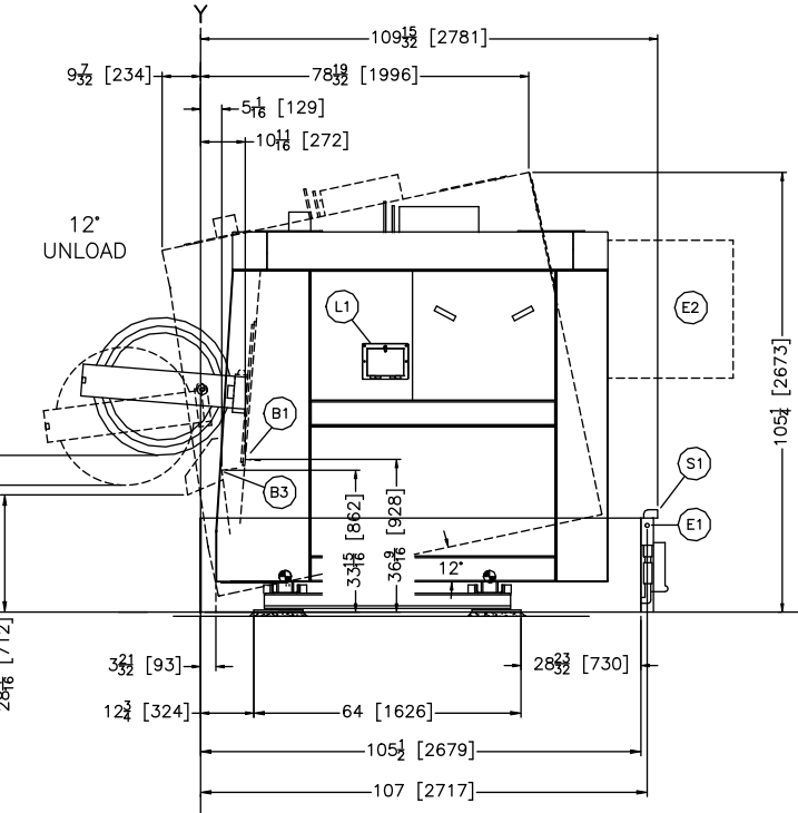
RIGHT VIEW
