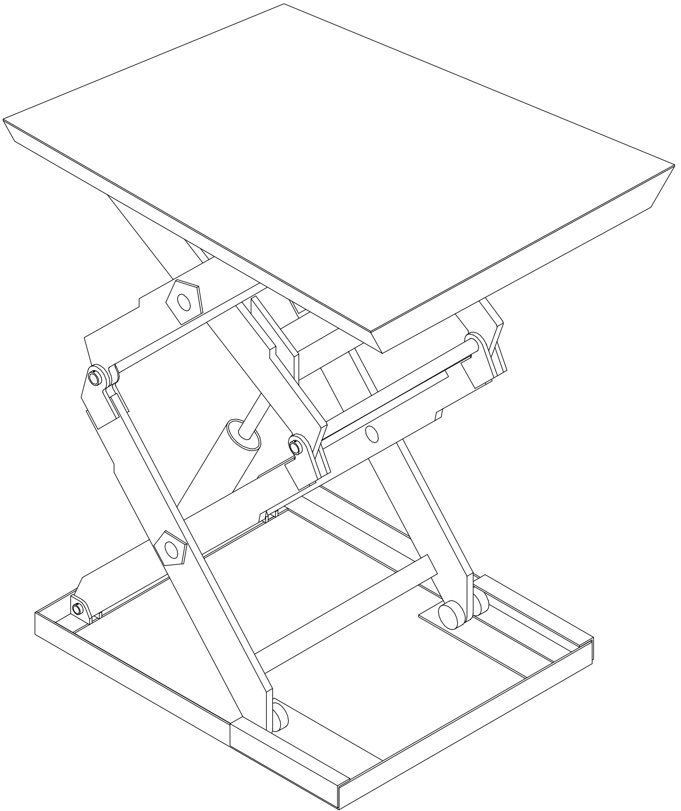
DSL-SERIES DOUBLE SCISSOR LIFT TABLE
