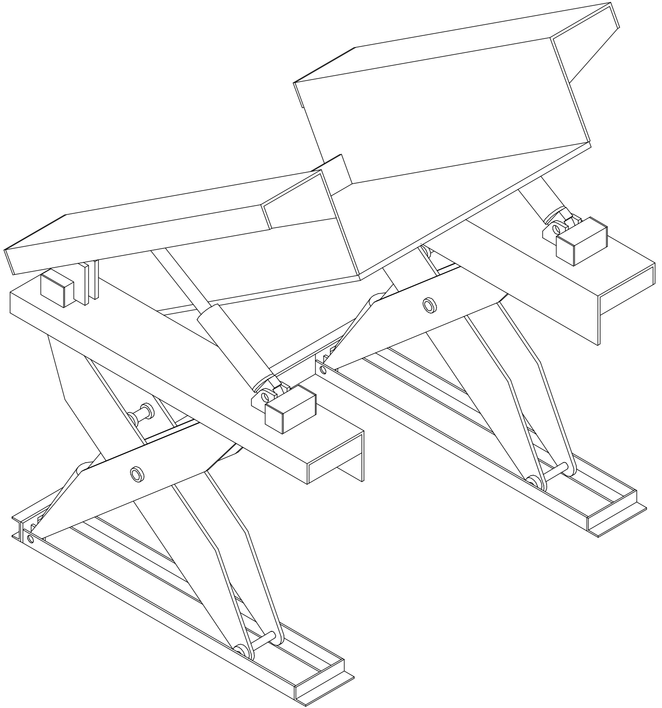
NO—LOW SERIES LIFT & TILT TABLE
