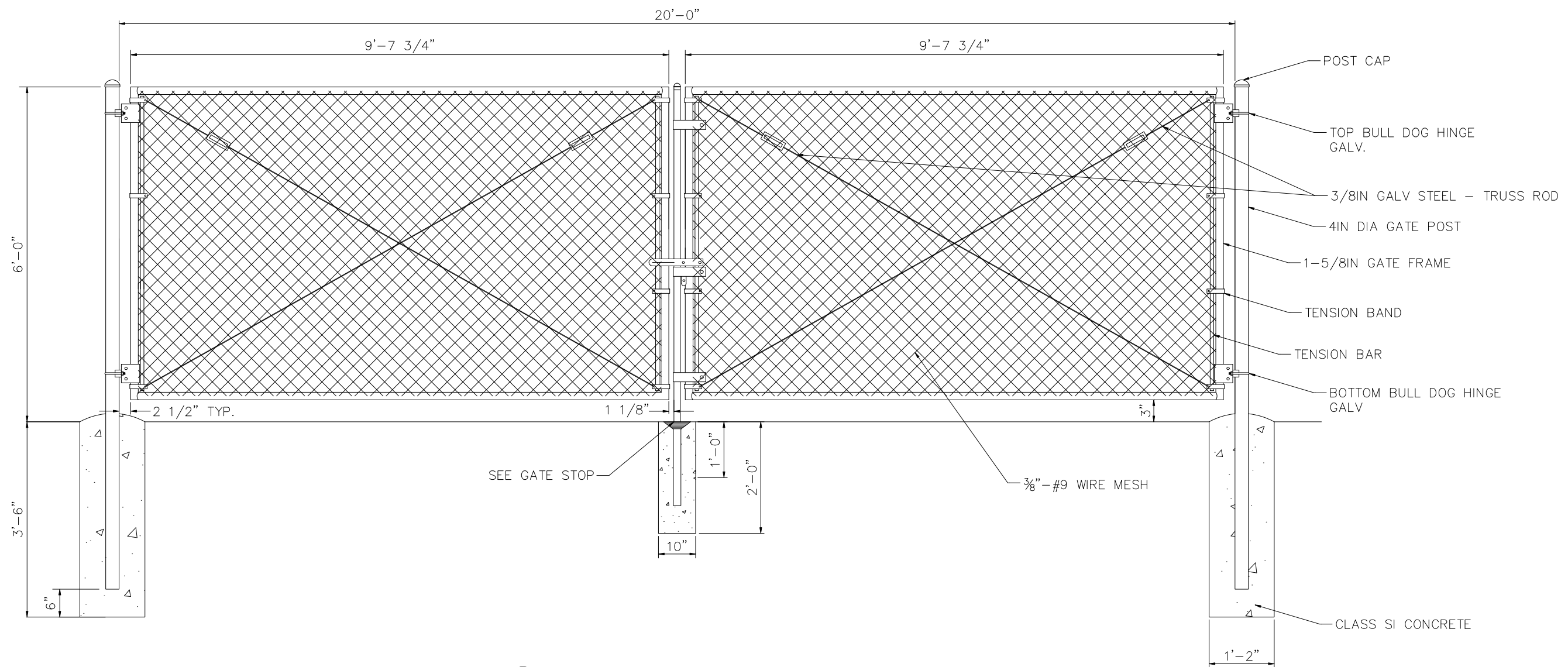
1 DOUBLE SWING GATE ELEVATION SCALE: NTS
