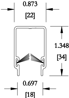
STANDARD SIDE TRACK c/w MESH RETENTION
