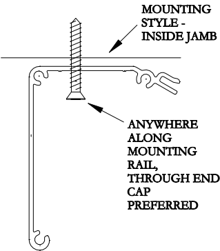
MOUNTING SCENARIO FOR THE HOUSING MOUNTING BRACKET (RAIL)
