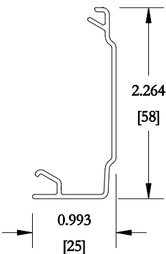
HOUSING COVER
