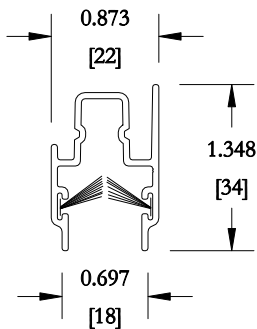
REMOVABLE TRACK c/w MESH RETENTION
