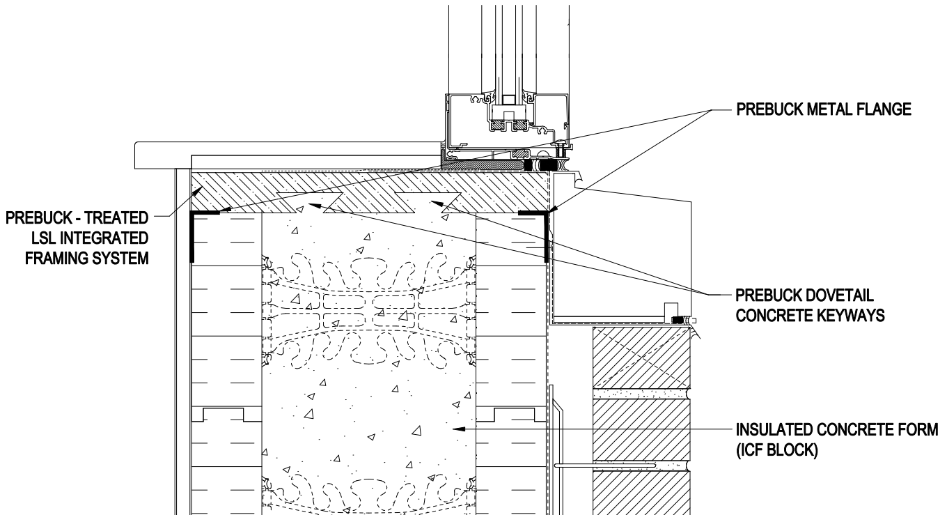
SECTION
