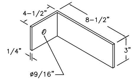
BRACKET DETAIL
