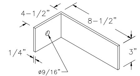
BRACKET DETAIL
