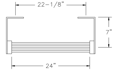
PLAN (SAFETY BARS OMITTED FOR CLARITY)
