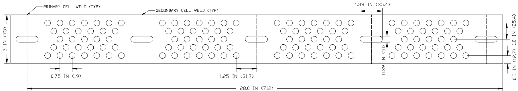
PERFORATION PATTERN – 3 IN (75 MM) COLLAPSED GEOWEB GW40V SECTIONS
