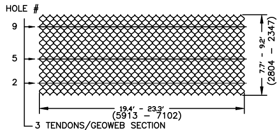
3 TENDON SPACING
