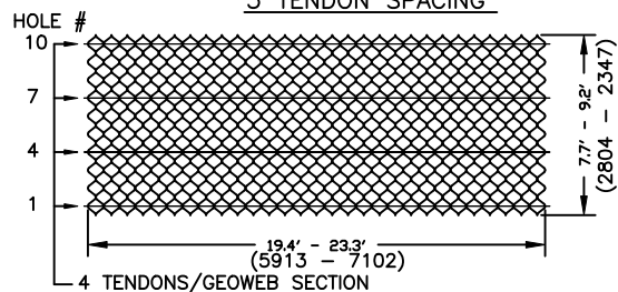
4 TENDON SPACING
