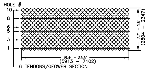
6 TENDON SPACING
