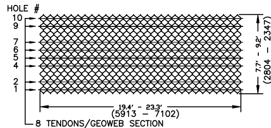
8 TENDON SPACING
