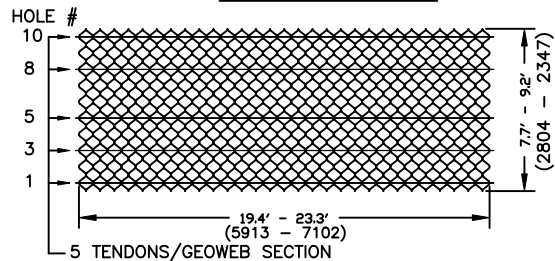
5 TENDON SPACING
