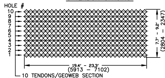
10 TENDON SPACING
