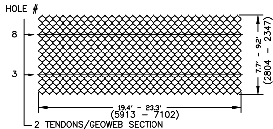
2 TENDON SPACING
