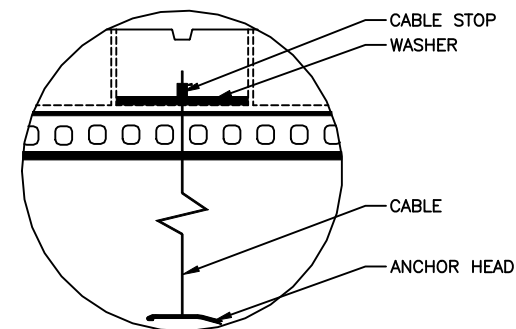
EARTH ANCHOR DETAIL
