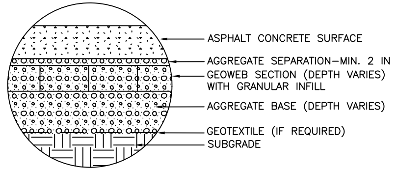
DETAIL B
