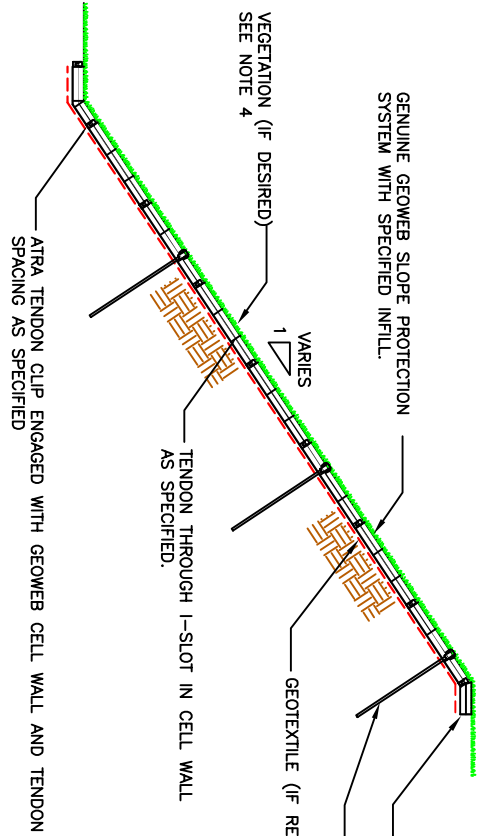
TYPICAL TENDON AND STAKE ANCHOR SYSTEM
