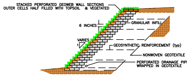
REINFORCED SLOPE - STACKED GEOWEB® FASCIA
