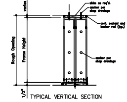
TYPICAL VERTICAL SECTION
