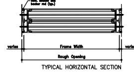
TYPICAL HORIZONTAL SECTION
