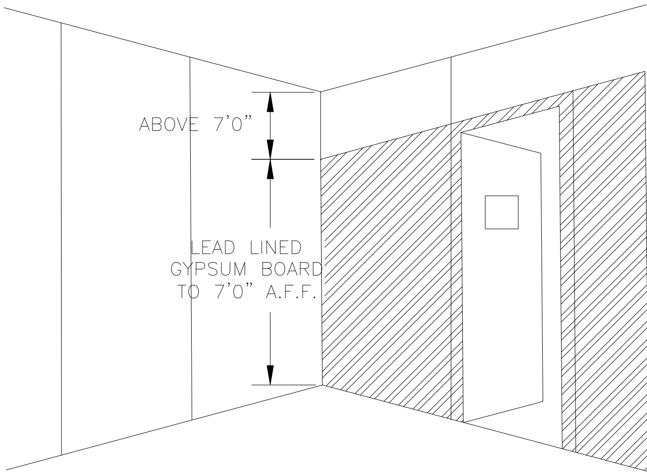
LEAD HEIGHT DETAIL NOT TO SCALE
