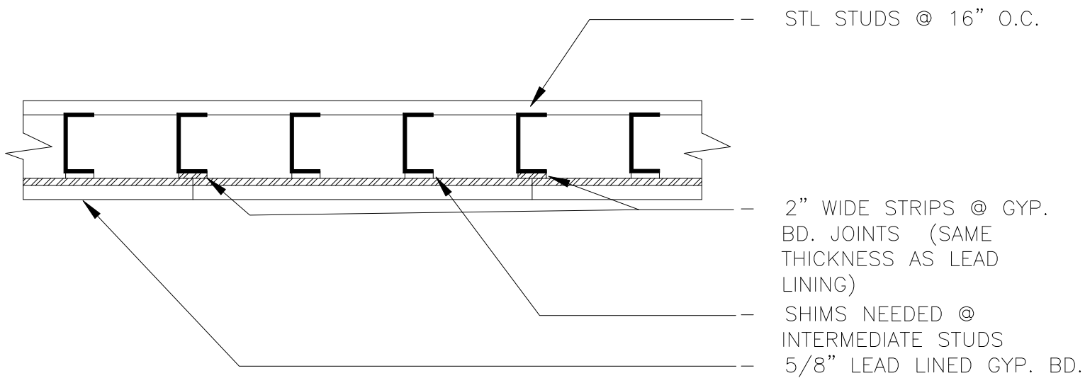
WALL DETAIL NOT TO SCALE
