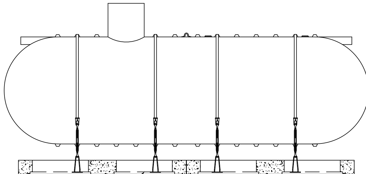
Deadman Detail Side View Note: Size of dead men and number of straps determined by tank size.
