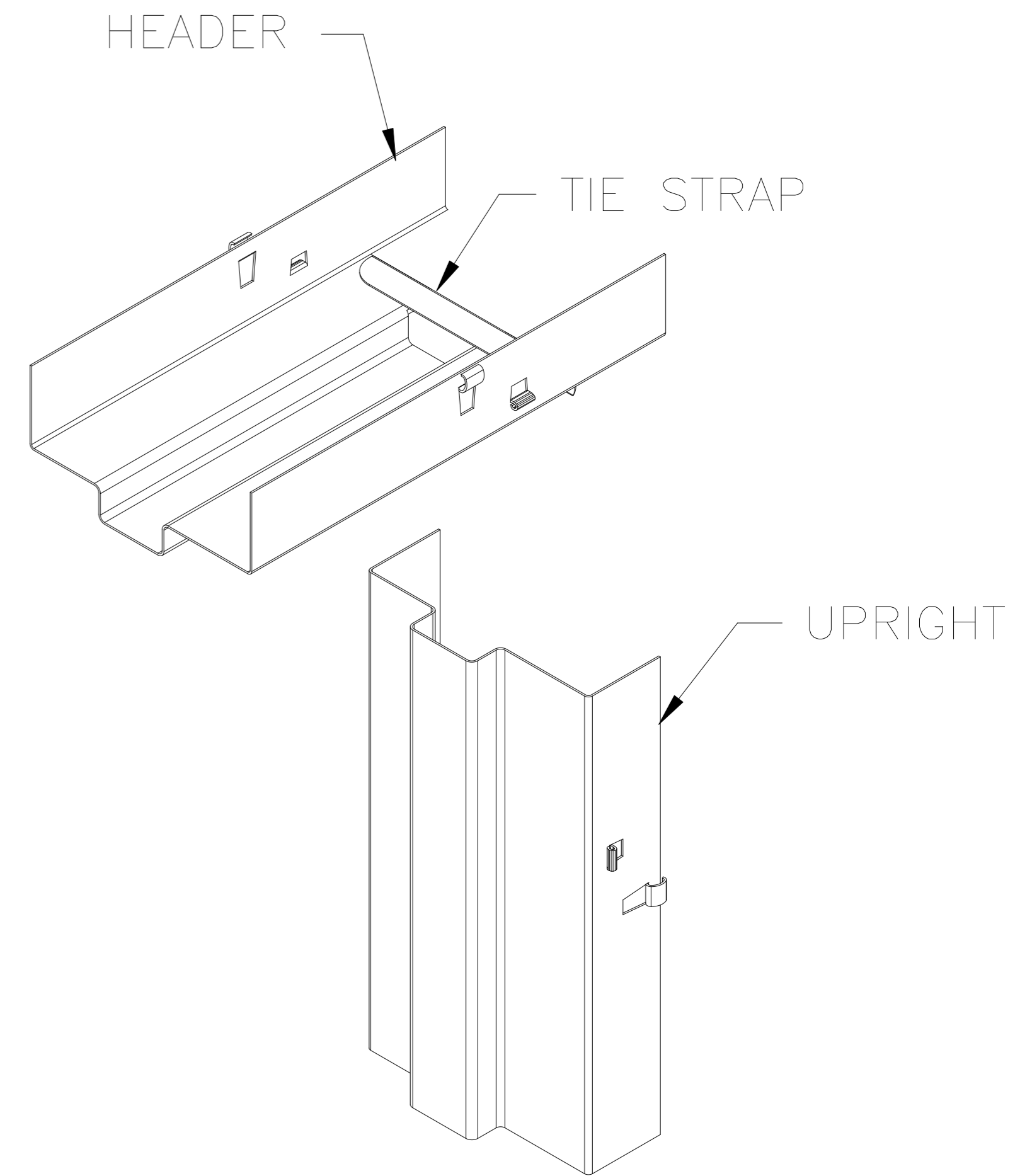
REDIFRAME CORNER DETAIL
