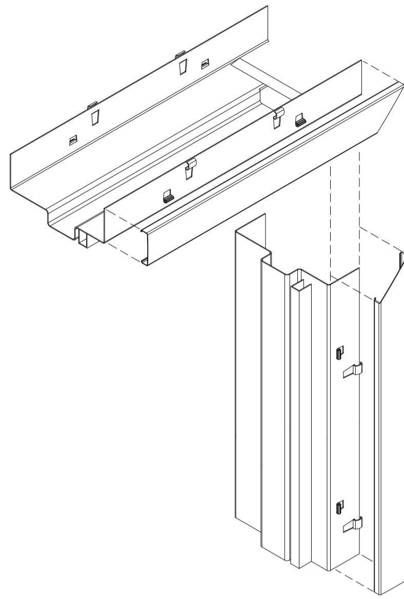
CORNER DETAIL WITH GLAZING BEAD
