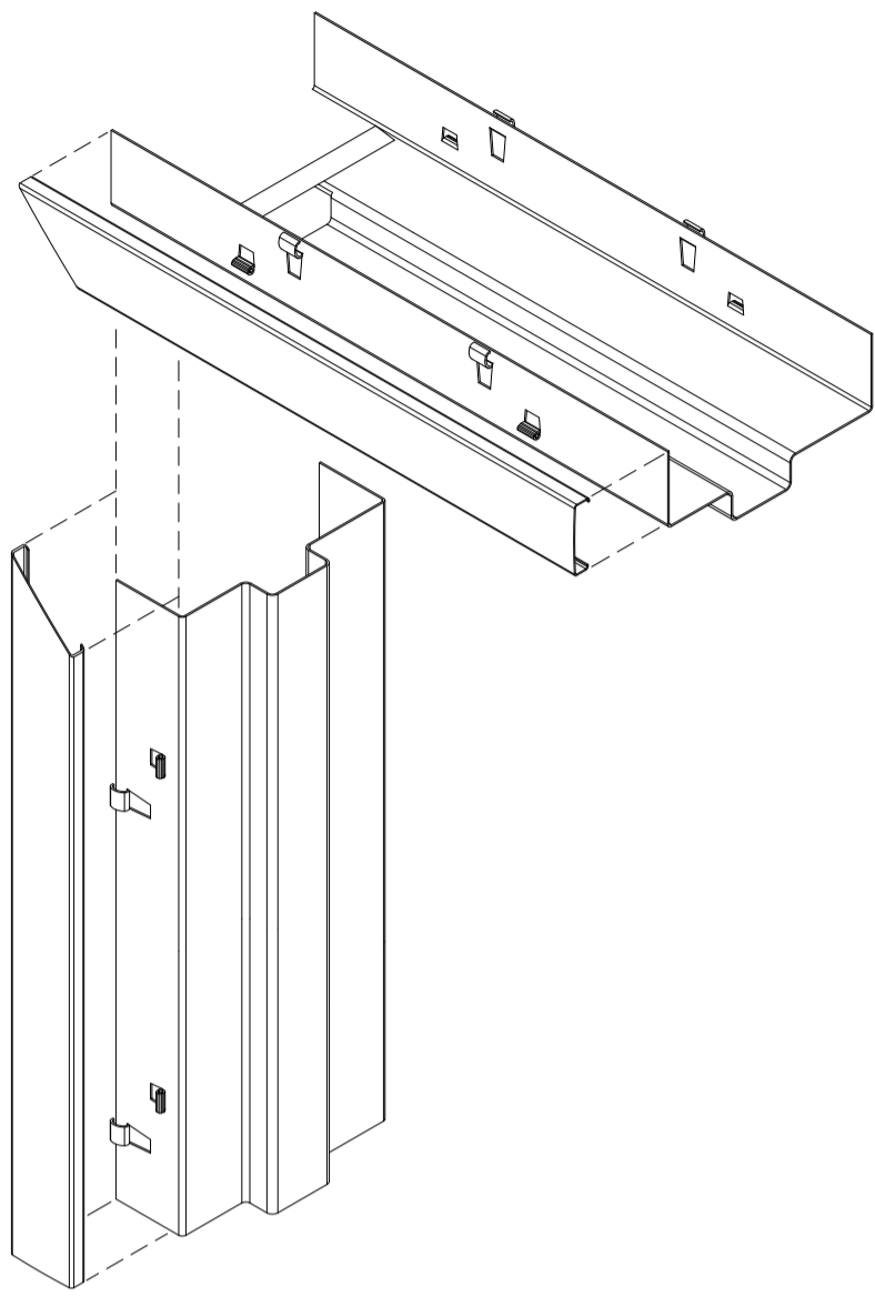
CORNER DETAIL
