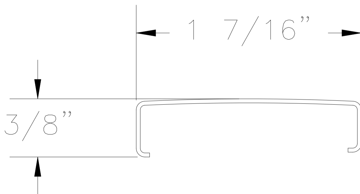
STEEL CASING
