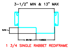
1 3/4 SINGLE RABBET REDIFRAME
