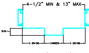
1 3/4 - 1 3/4 COMMUNICATING EQUAL RABBET REDIFRAME
