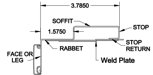
STANDARD 1-3/8" DOOR BASE
