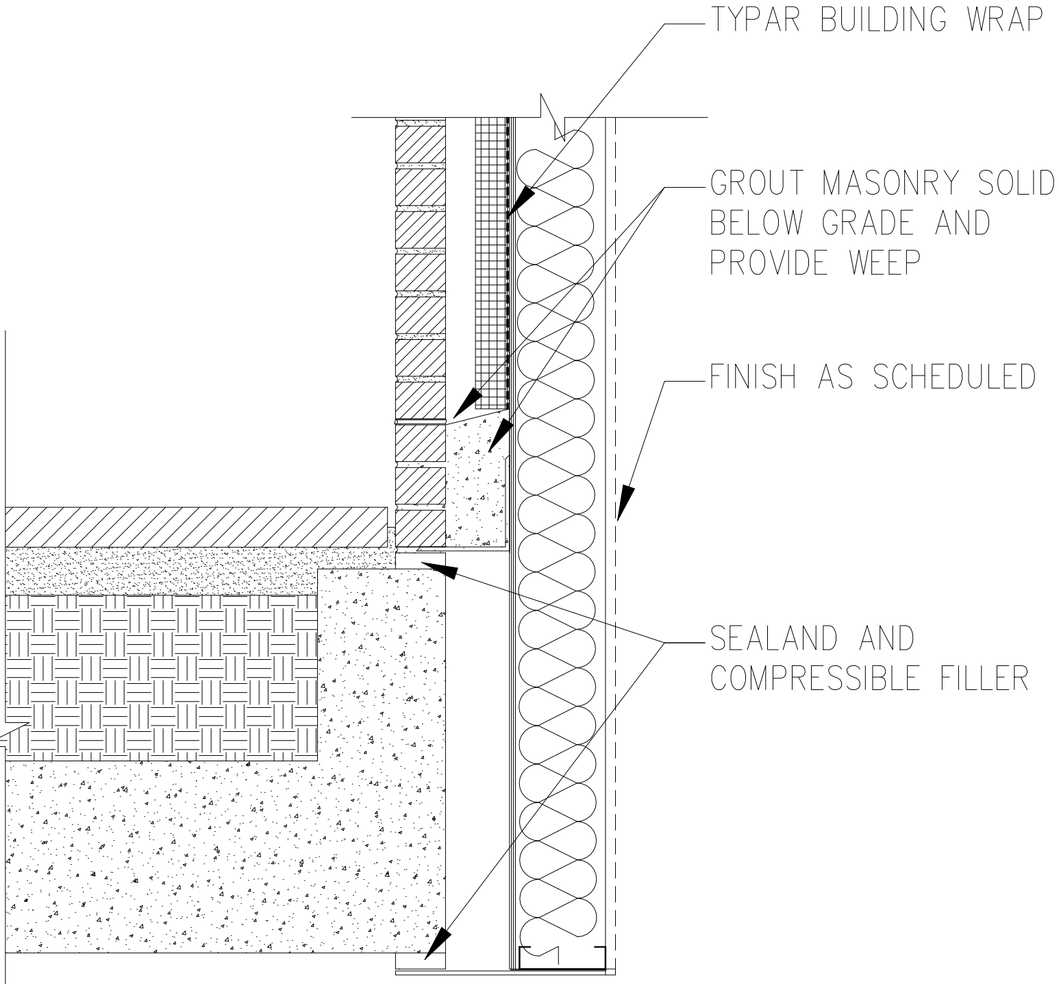
TYPICAL DETAIL @ ELEVATED TERRACE
