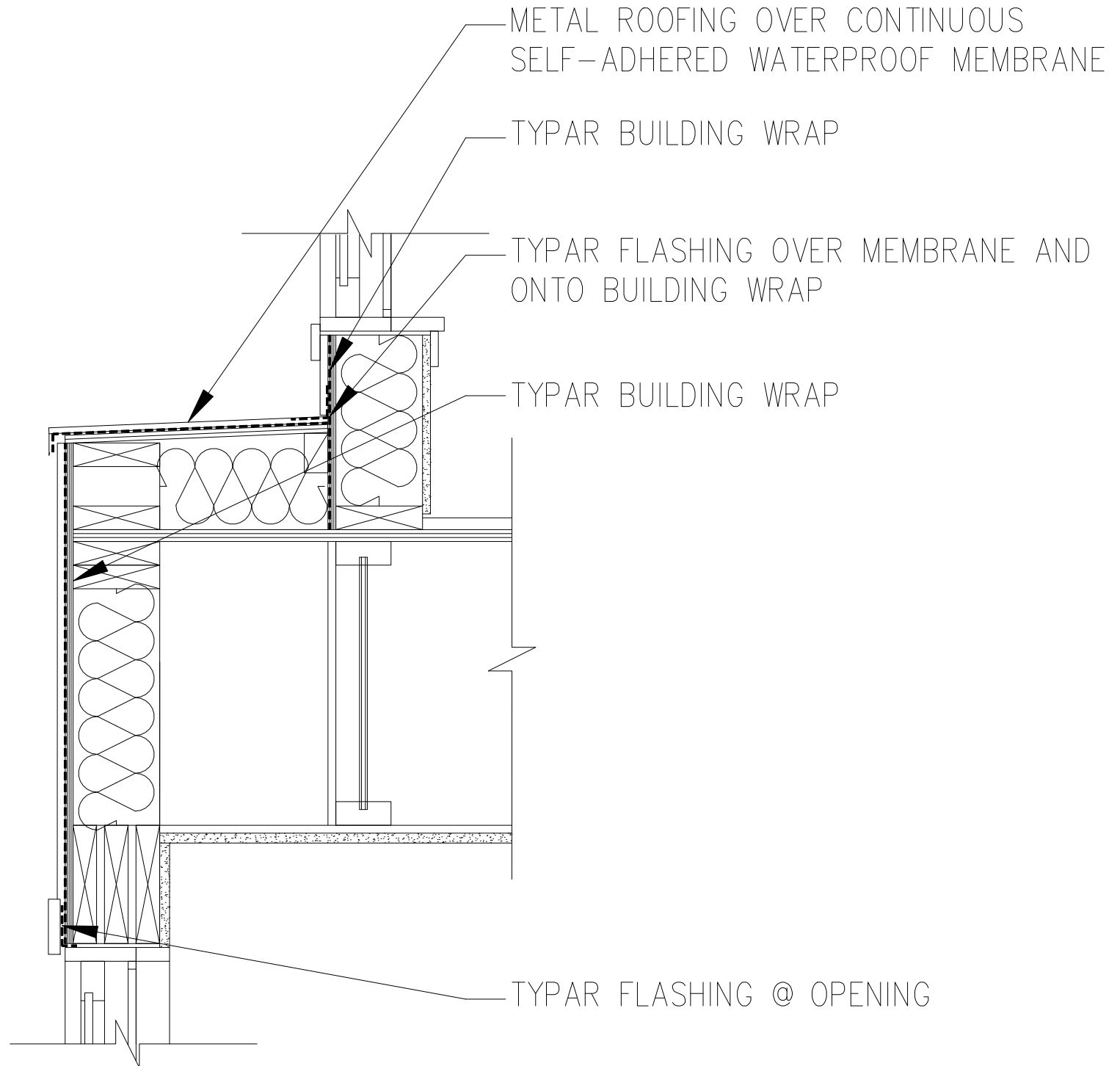
TYPICAL LOW-SLOPE ROOF TRANSITION DETAIL
