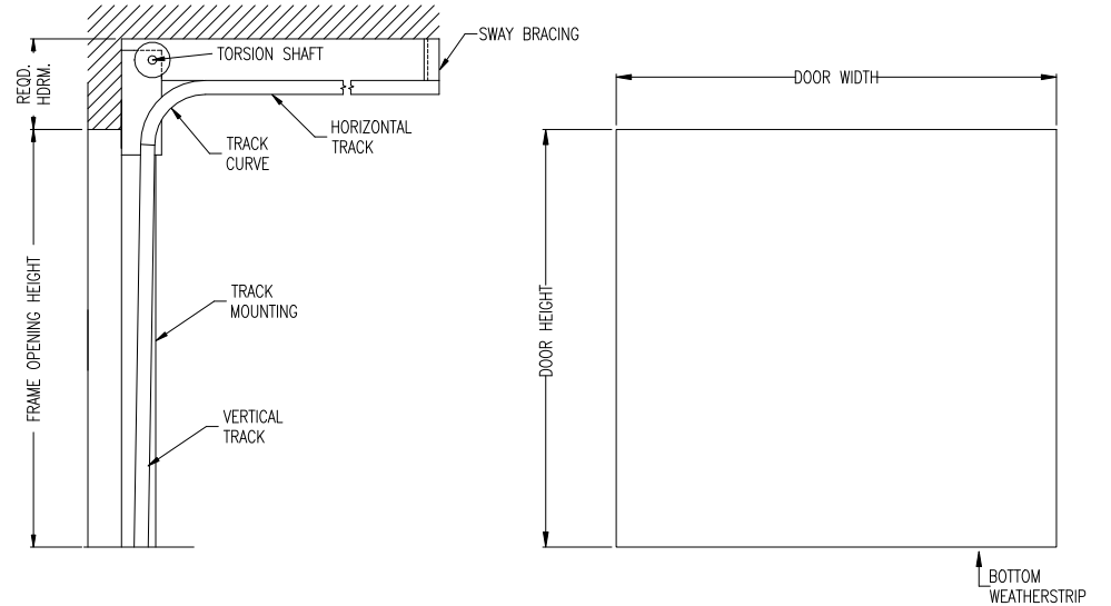
CROSS SECTION
