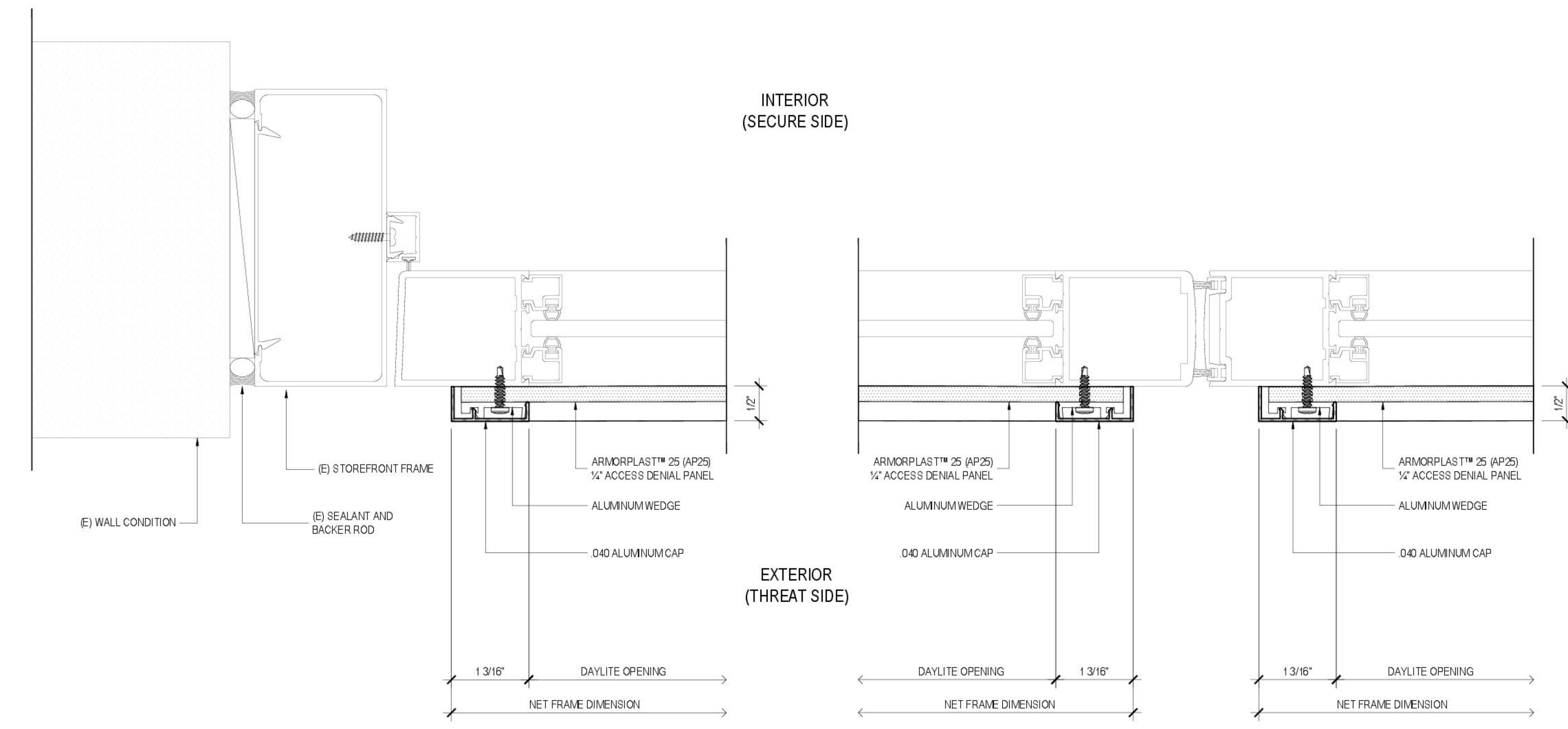
107 (SURFACE MOUNT) STOREFRONT DOOR JAMB DETAIL 604 ARCHITECTURAL REF
