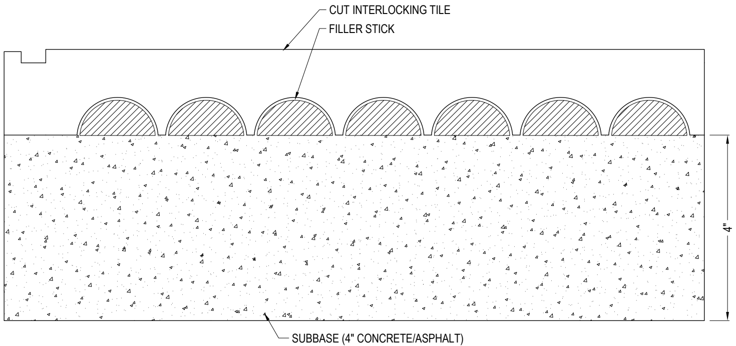
SECTION VIEW TILE WITH FILLER STICK
